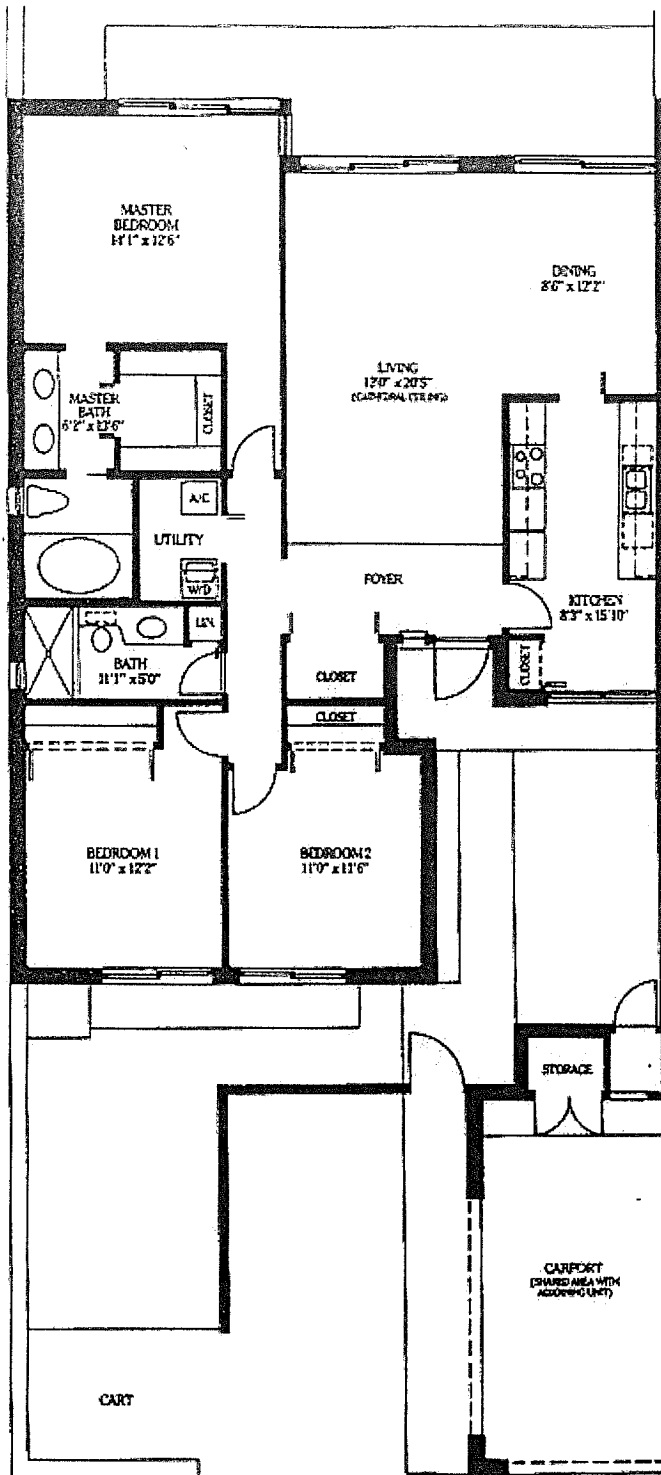
CAPE POINTE - UNIT A
