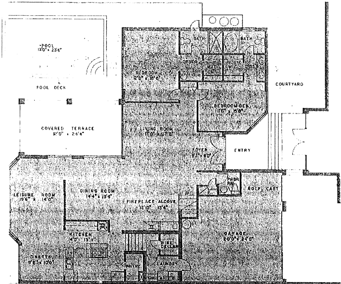
UNIT C--FIRST FLOOR
